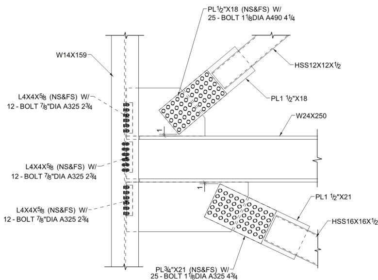
BF-1 ELEVATION ALONG GL A
